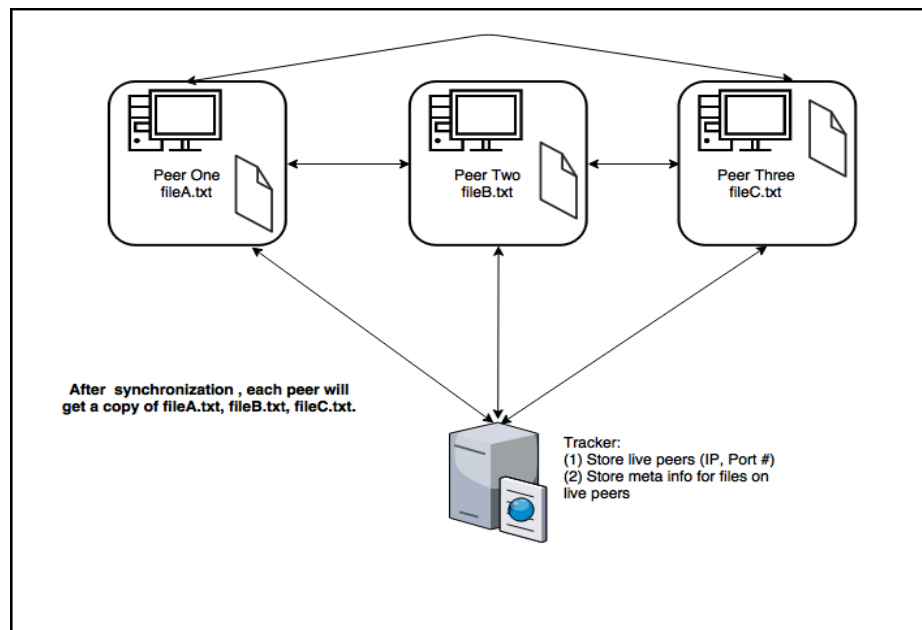
Figure 1 P2P file sharing architecture
